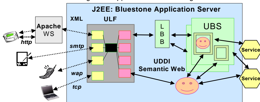
Figure 8: Appliances + J2EE + Agents
